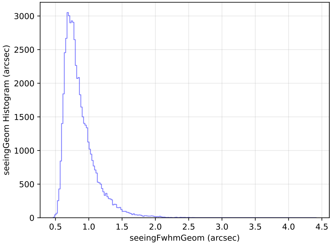
too_ignore_5_1v3.4_10yrs Yr 1 i band: seeingGeom Histogram
