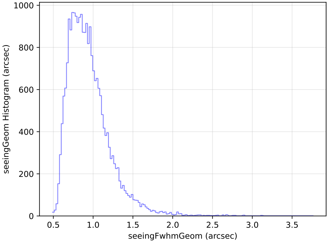
too_ignore_5_1v3.4_10yrs Yr 1 g band: seeingGeom Histogram
