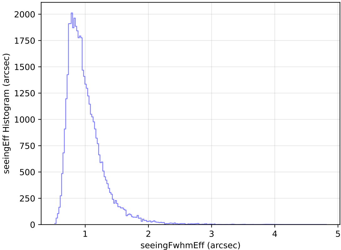
too_ignore_5_1v3.4_10yrs Yr 1 z band: seeingEff Histogram
