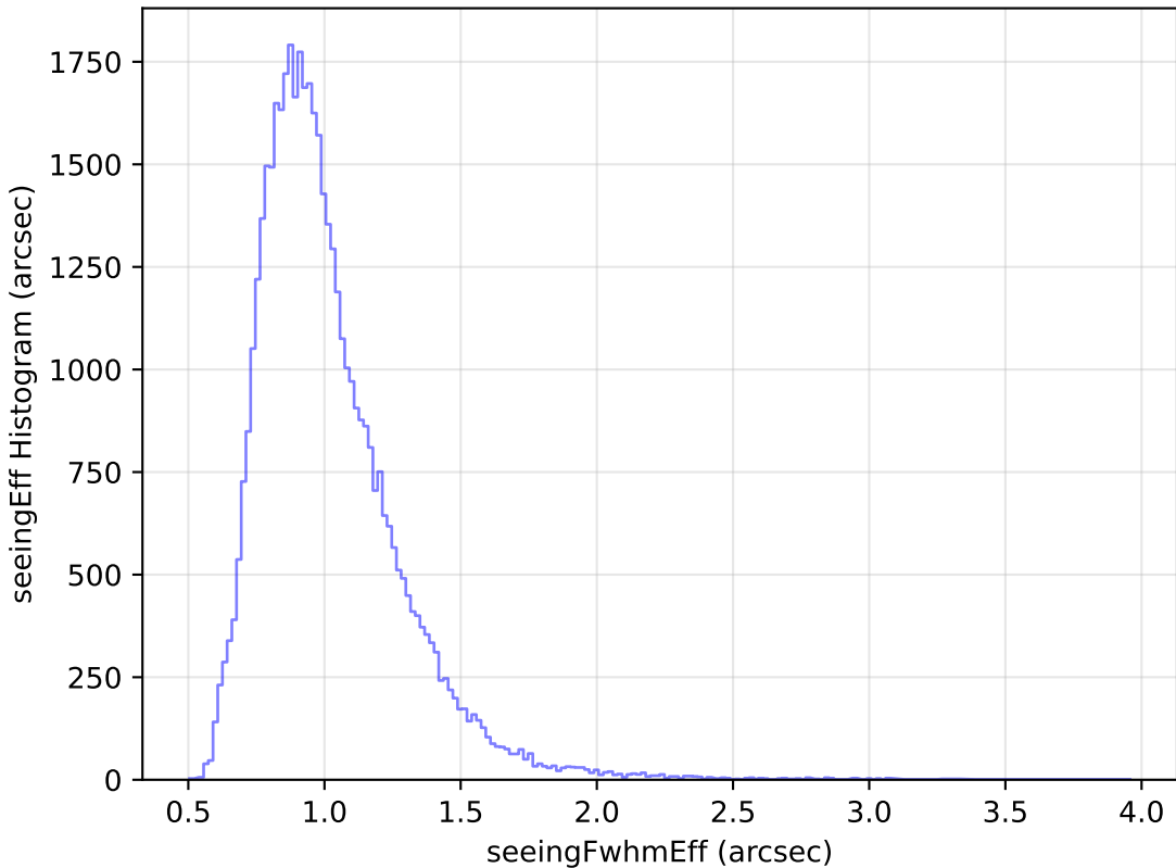
too_ignore_5_1v3.4_10yrs Yr 1 y band: seeingEff Histogram
