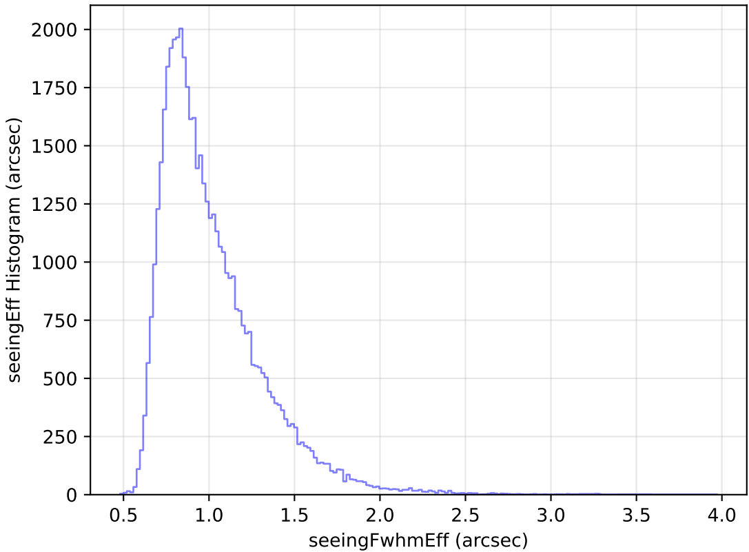
too_ignore_5_1v3.4_10yrs Yr 1 r band: seeingEff Histogram
