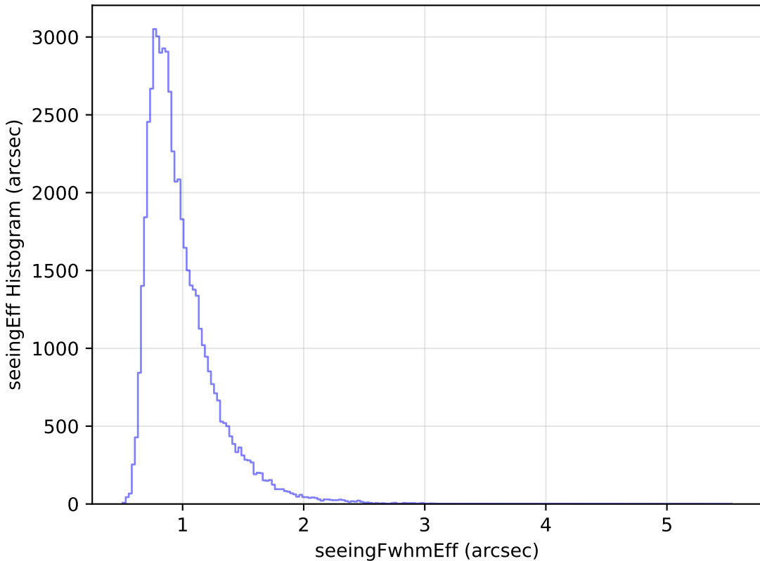
too_ignore_5_1v3.4_10yrs Yr 1 i band: seeingEff Histogram
