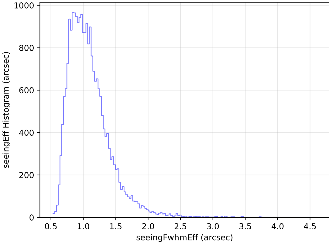
too_ignore_5_1v3.4_10yrs Yr 1 g band: seeingEff Histogram
