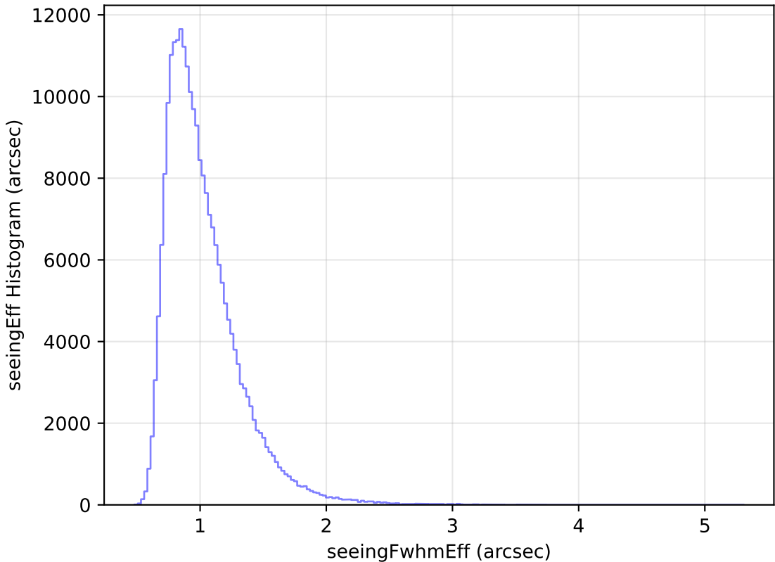
too_ignore_5_1v3.4_10yrs Yr 1 all bands: seeingEff Histogram
