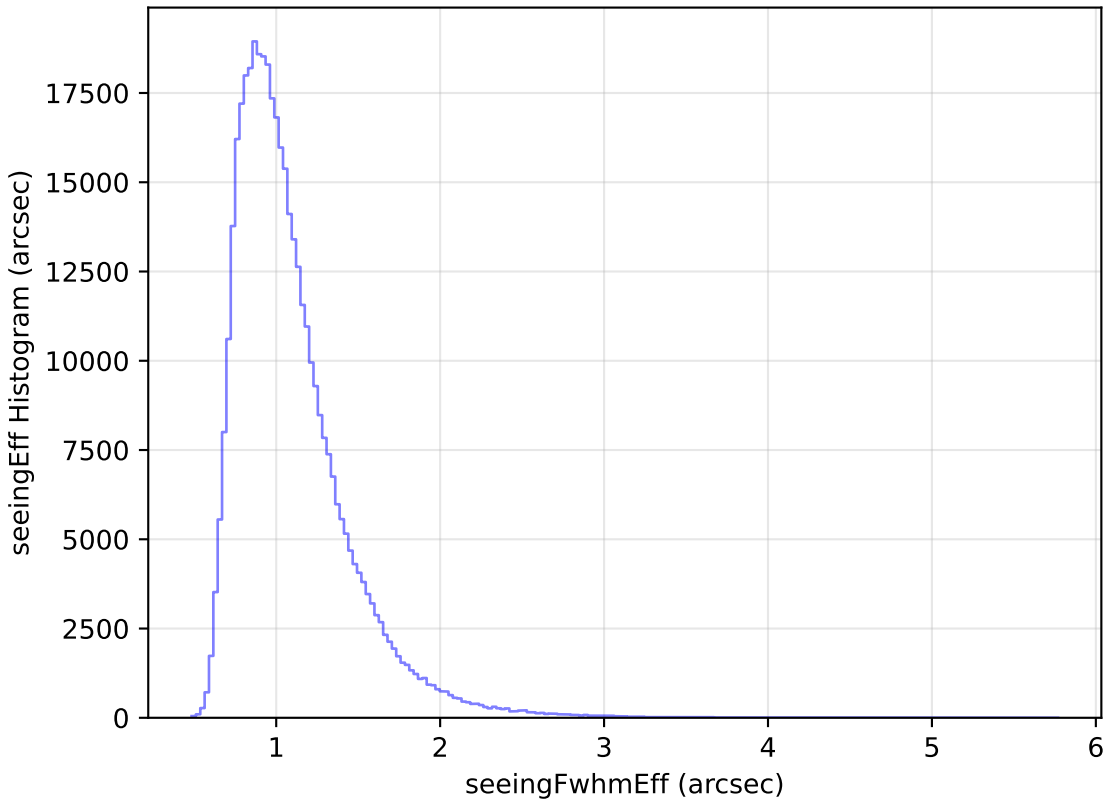
too_ignore_5_1v3.4_10yrs WFD z band: seeingEff Histogram
