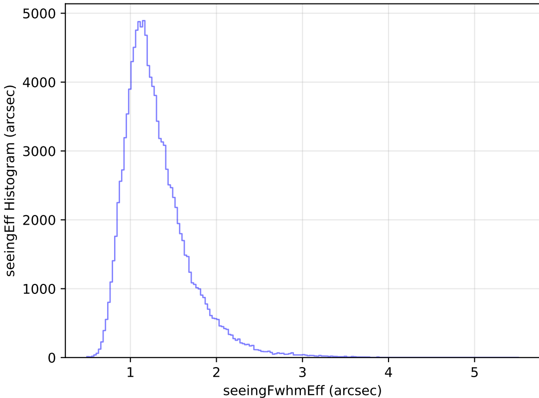
too_ignore_5_1v3.4_10yrs WFD u band: seeingEff Histogram
