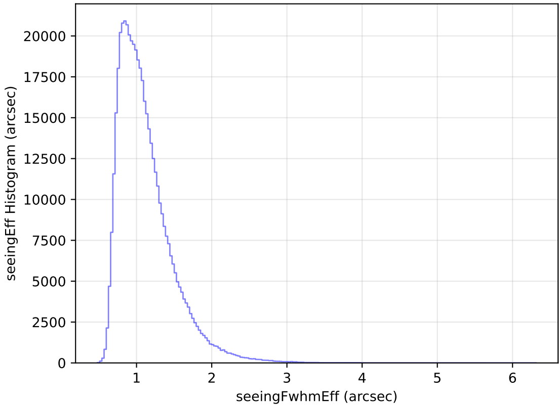
too_ignore_5_1v3.4_10yrs WFD r band: seeingEff Histogram
