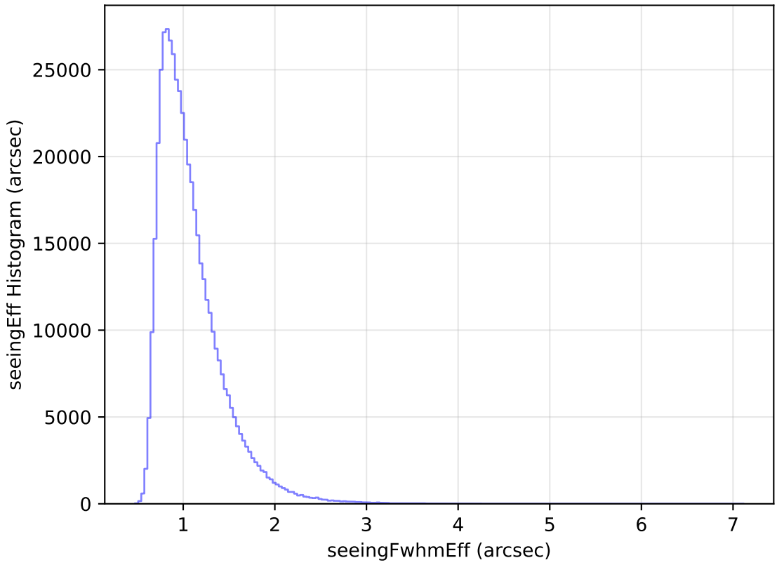
too_ignore_5_1v3.4_10yrs WFD i band: seeingEff Histogram
