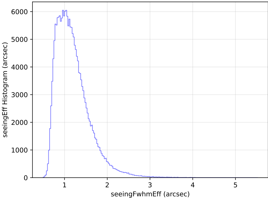
too_ignore_5_1v3.4_10yrs WFD g band: seeingEff Histogram
