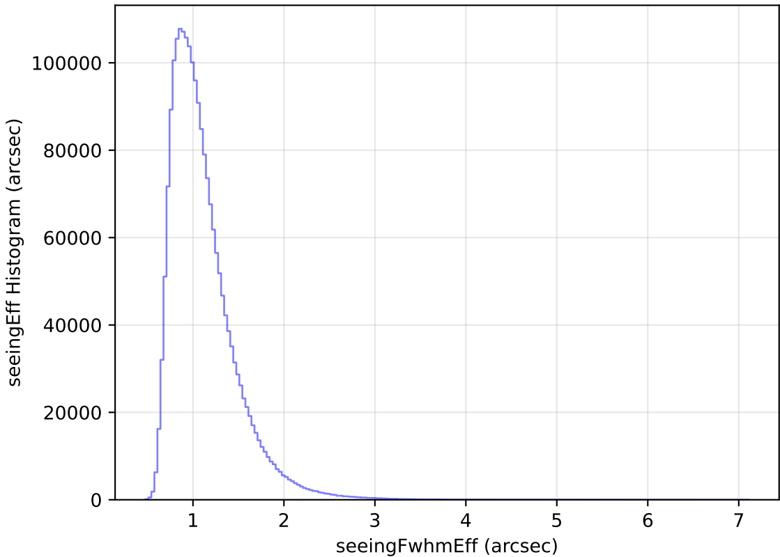
too_ignore_5_1v3.4_10yrs WFD all bands: seeingEff Histogram
