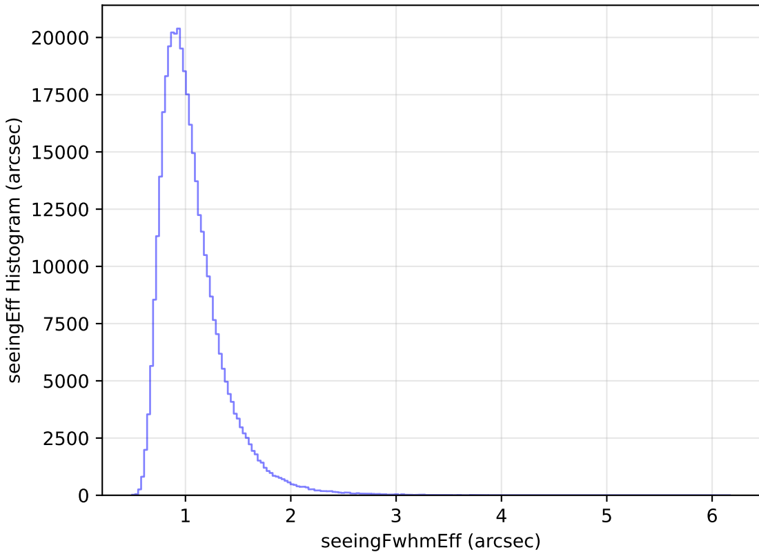
too_ignore_5_1v3.4_10yrs All sky y band: seeingEff Histogram
