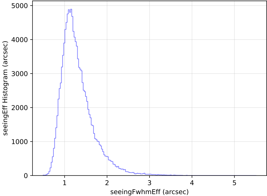
too_ignore_5_1v3.4_10yrs All sky u band: seeingEff Histogram
