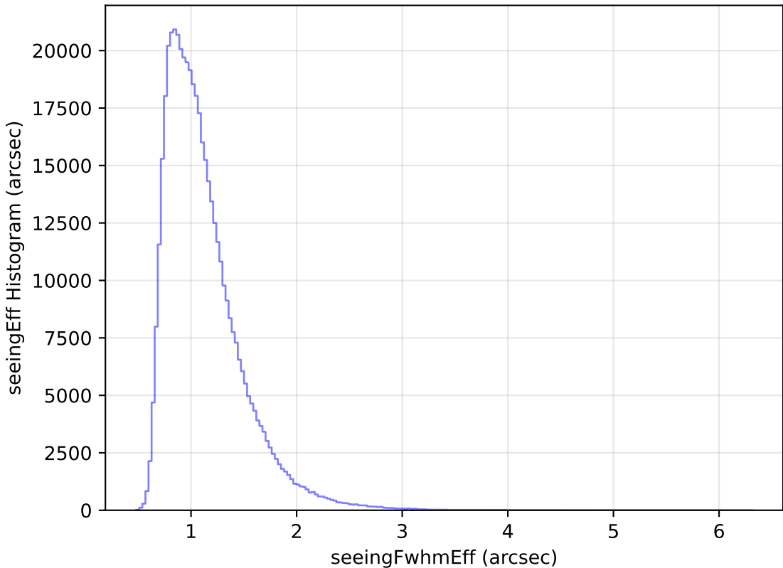
too_ignore_5_1v3.4_10yrs All sky r band: seeingEff Histogram
