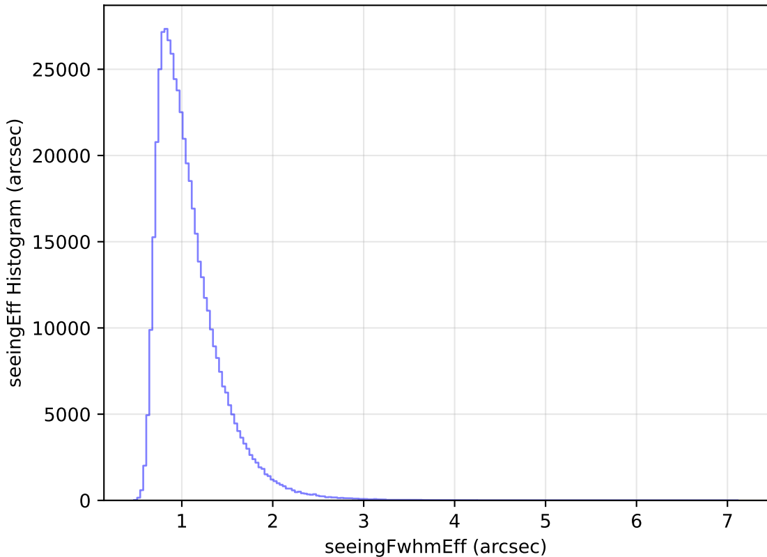
too_ignore_5_1v3.4_10yrs All sky i band: seeingEff Histogram
