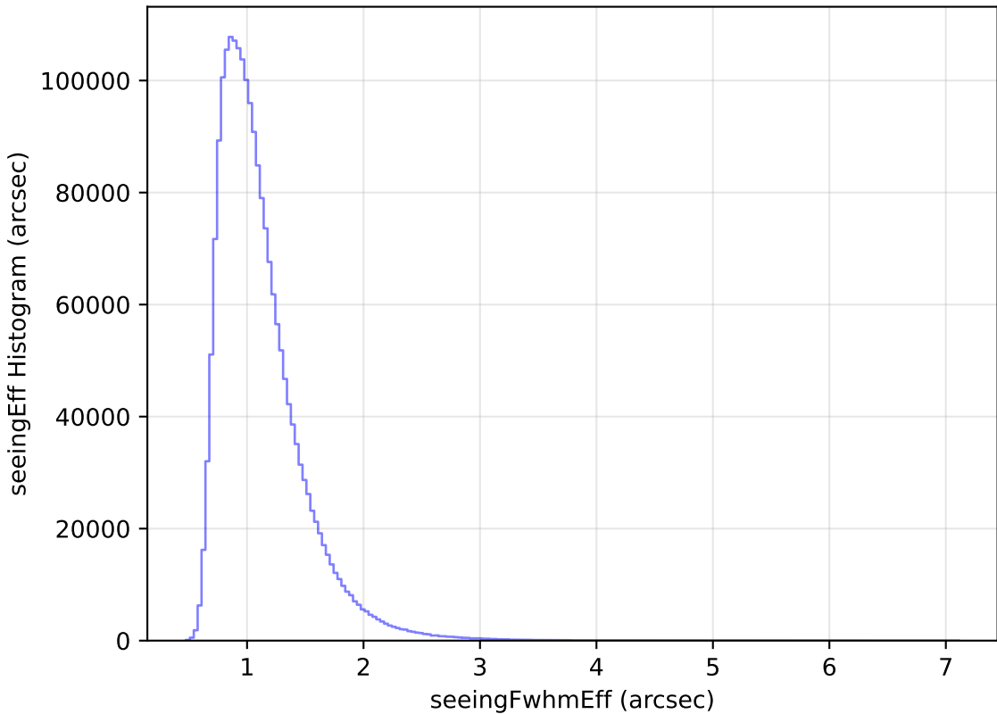
too_ignore_5_1v3.4_10yrs All sky all bands: seeingEff Histogram
