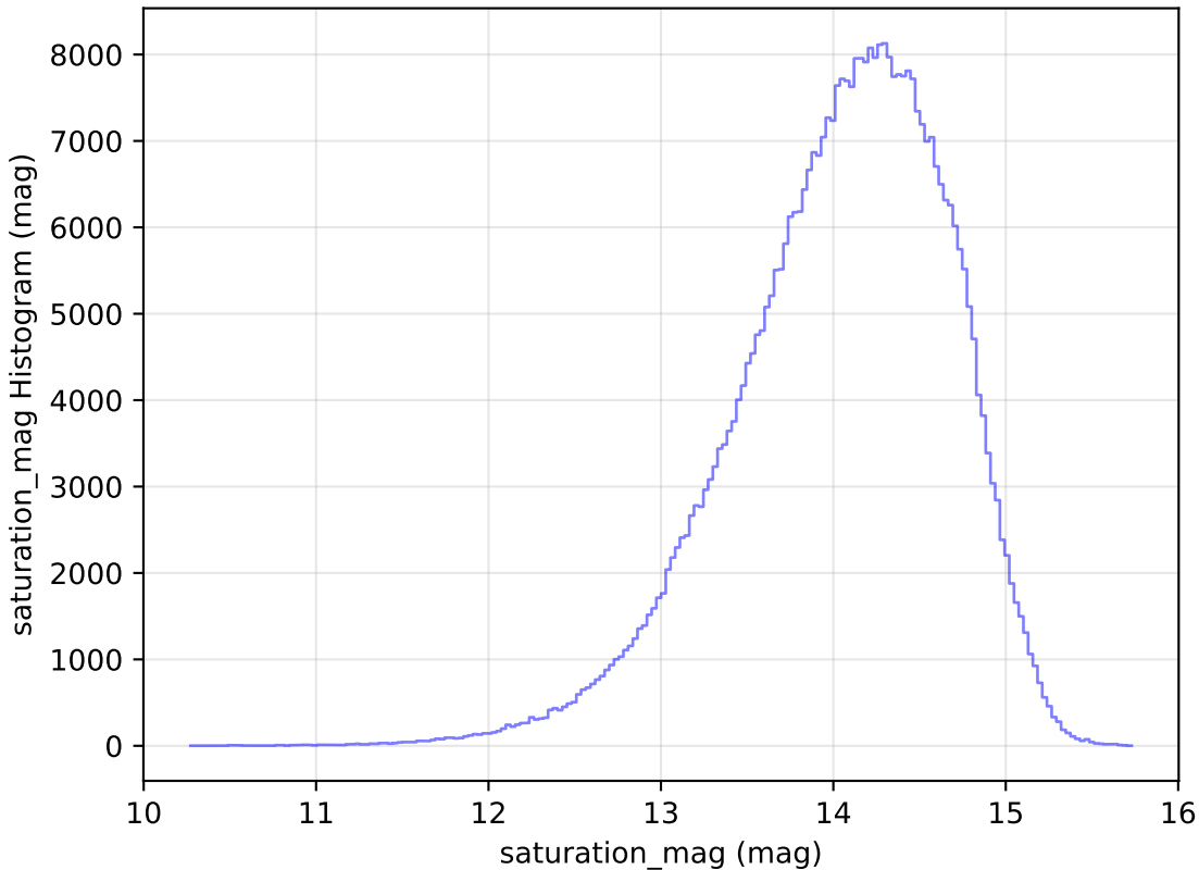
too_ignore_5_1v3.4_10yrs WFD z band: saturation_mag Histogram
