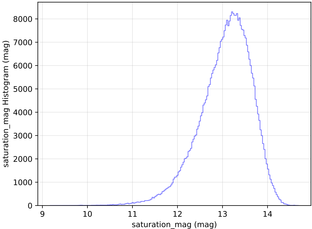
too_ignore_5_1v3.4_10yrs WFD y band: saturation_mag Histogram
