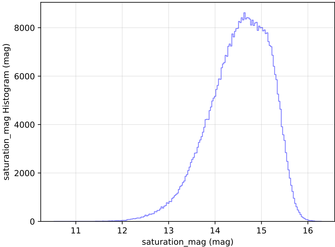
too_ignore_5_1v3.4_10yrs WFD r band: saturation_mag Histogram
