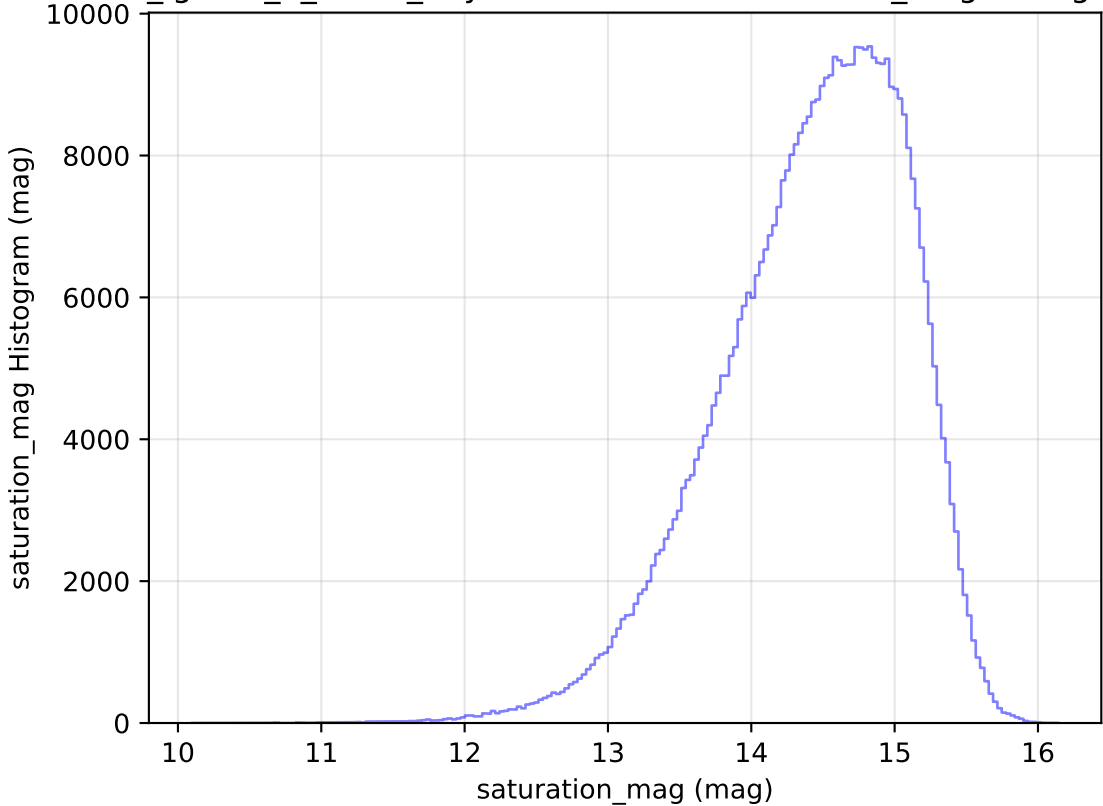
too_ignore_5_1v3.4_10yrs WFD i band: saturation_mag Histogram
