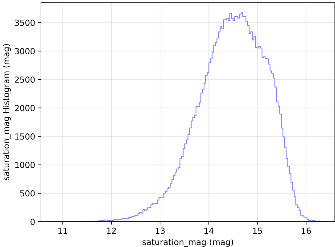
too_ignore_5_1v3.4_10yrs WFD g band: saturation_mag Histogram
