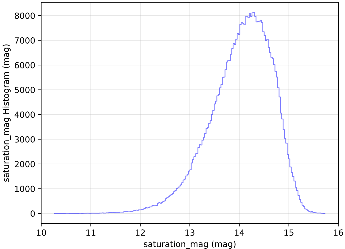
too_ignore_5_1v3.4_10yrs All sky z band: saturation_mag Histogram
