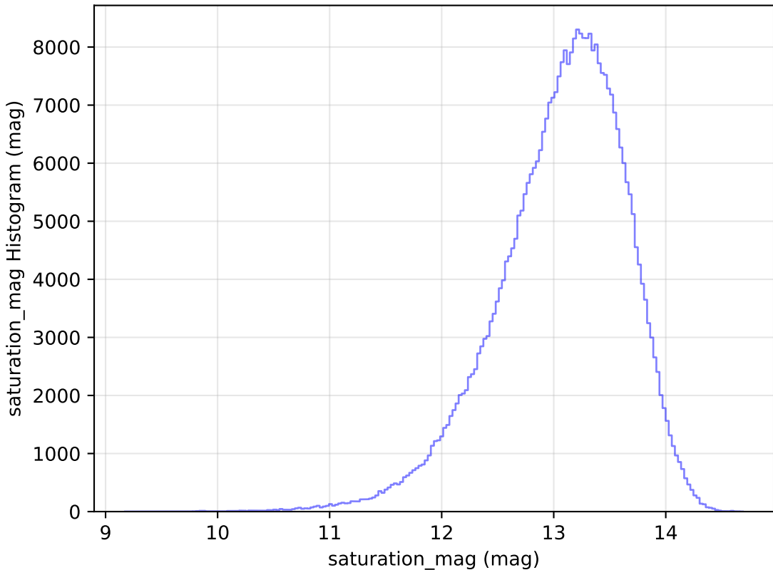
too_ignore_5_1v3.4_10yrs All sky y band: saturation_mag Histogram
