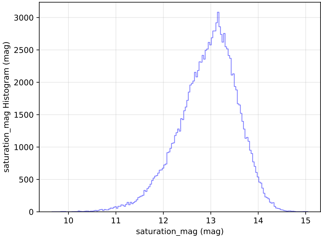
too_ignore_5_1v3.4_10yrs All sky u band: saturation_mag Histogram
