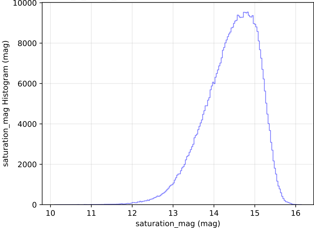
too_ignore_5_1v3.4_10yrs All sky i band: saturation_mag Histogram
