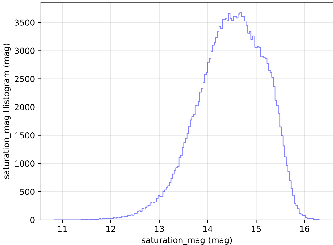
too_ignore_5_1v3.4_10yrs All sky g band: saturation_mag Histogram
