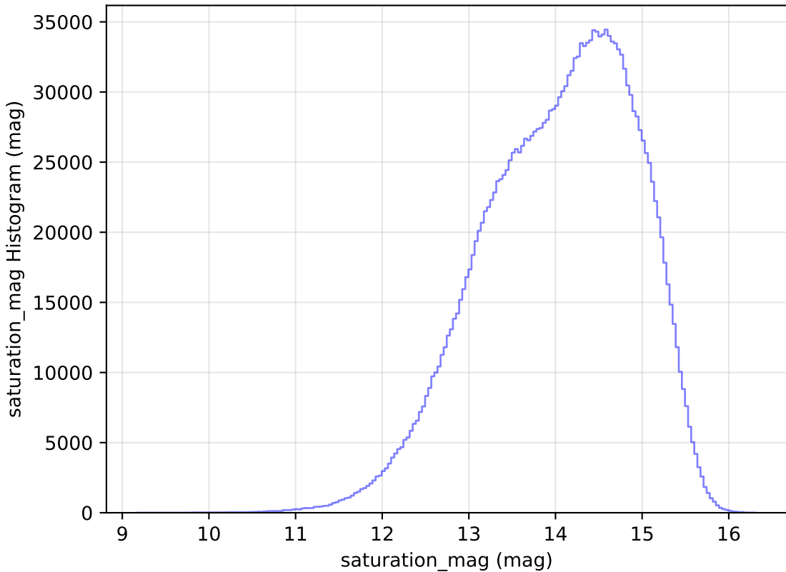
too_ignore_5_1v3.4_10yrs All sky all bands: saturation_mag Histogram
