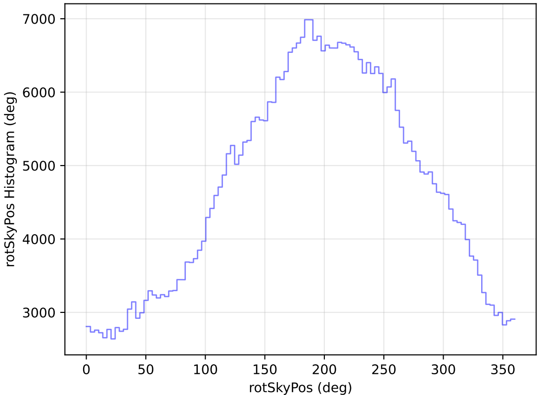
too_ignore_5_1v3.4_10yrs WFD r band: rotSkyPos Histogram
