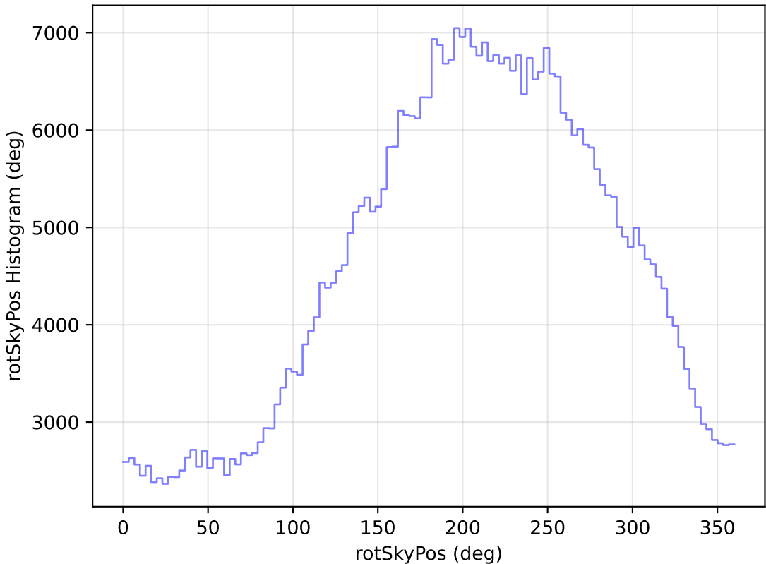
too_ignore_5_1v3.4_10yrs WFD i band: rotSkyPos Histogram
