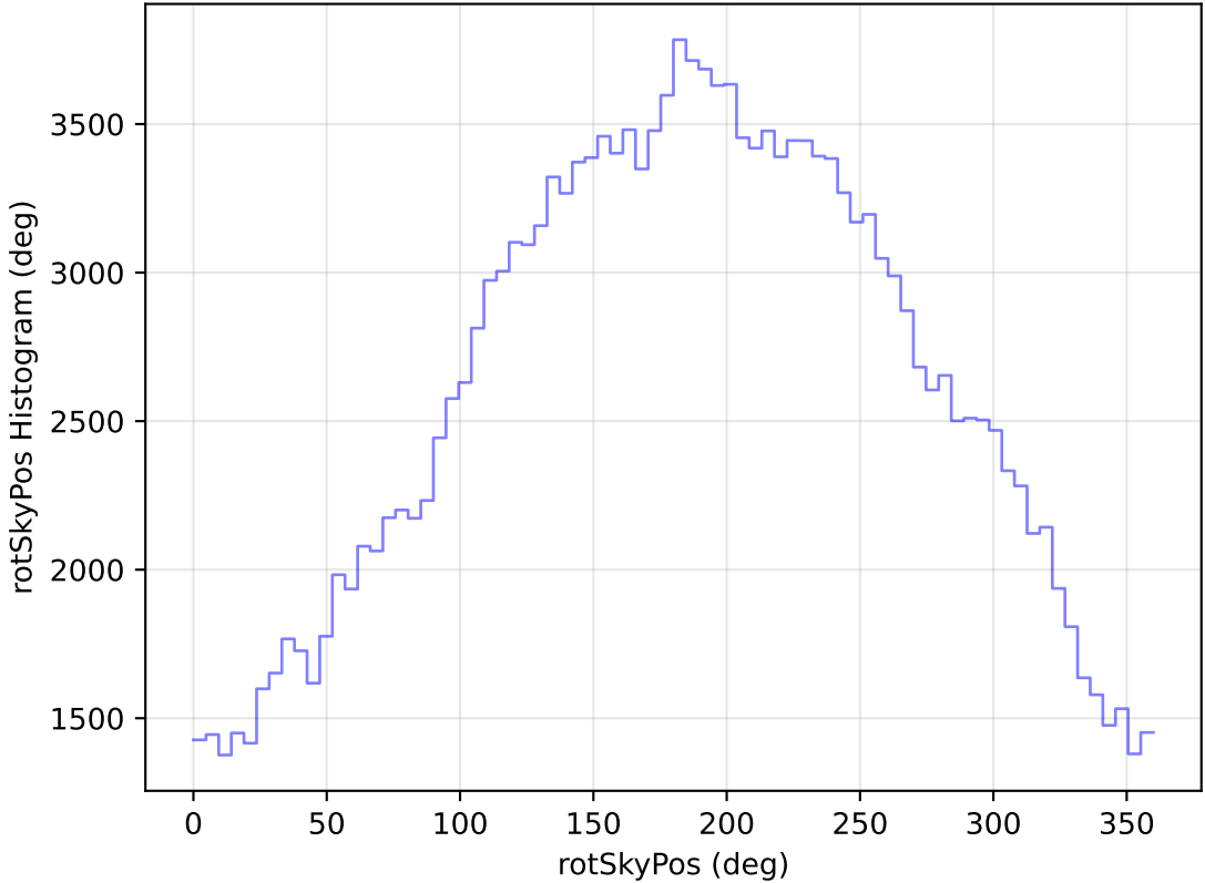
too_ignore_5_1v3.4_10yrs WFD g band: rotSkyPos Histogram
