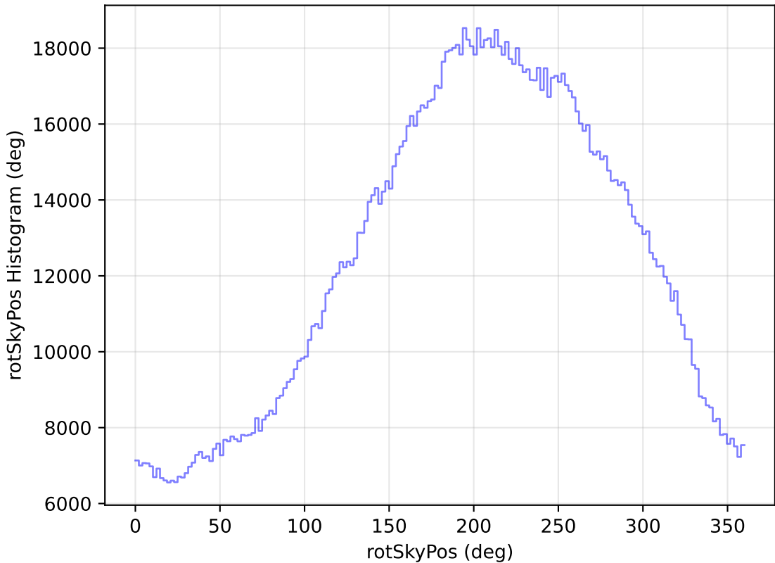
too_ignore_5_1v3.4_10yrs WFD all bands: rotSkyPos Histogram
