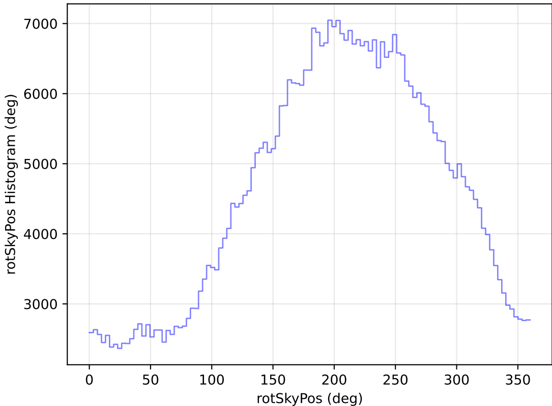
too_ignore_5_1v3.4_10yrs All sky i band: rotSkyPos Histogram
