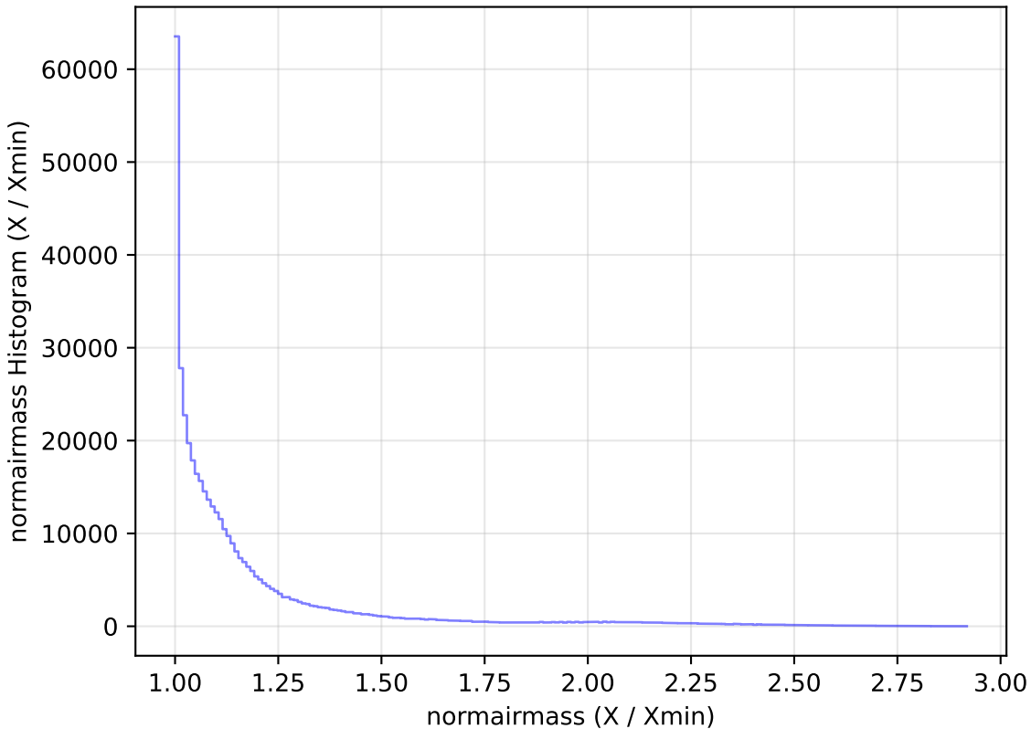
too_ignore_5_1v3.4_10yrs WFD z band: normairmass Histogram
