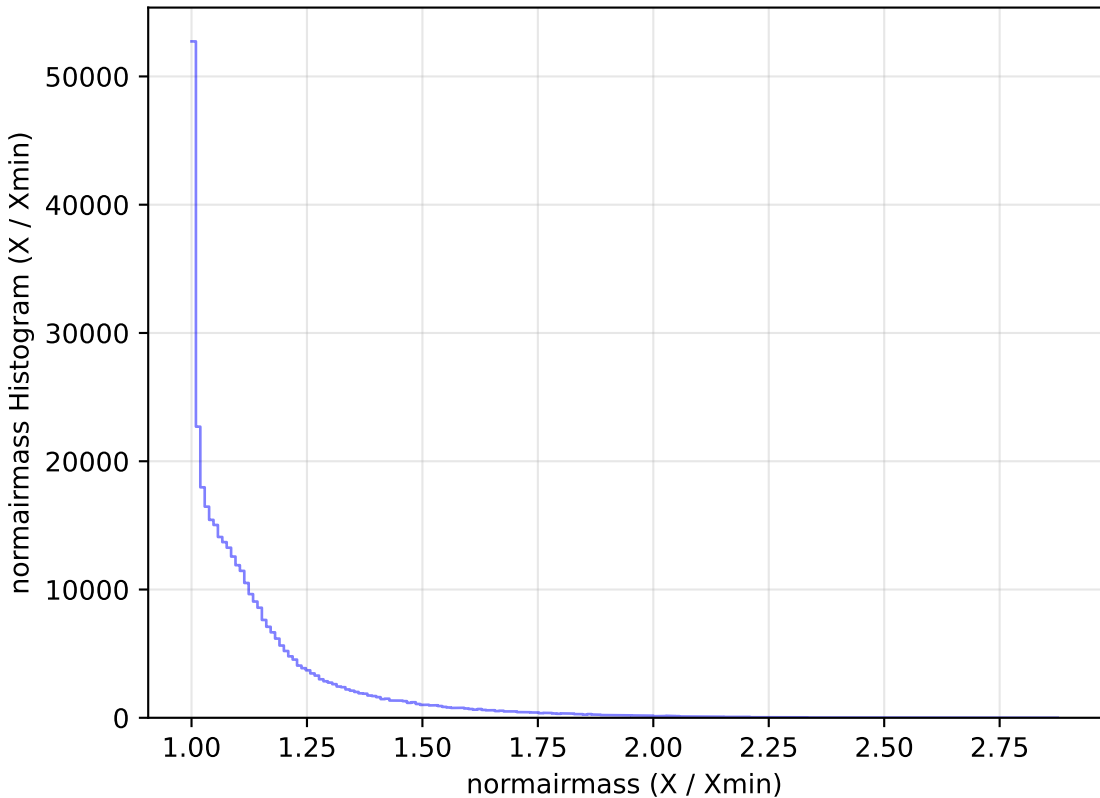
too_ignore_5_1v3.4_10yrs WFD y band: normairmass Histogram
