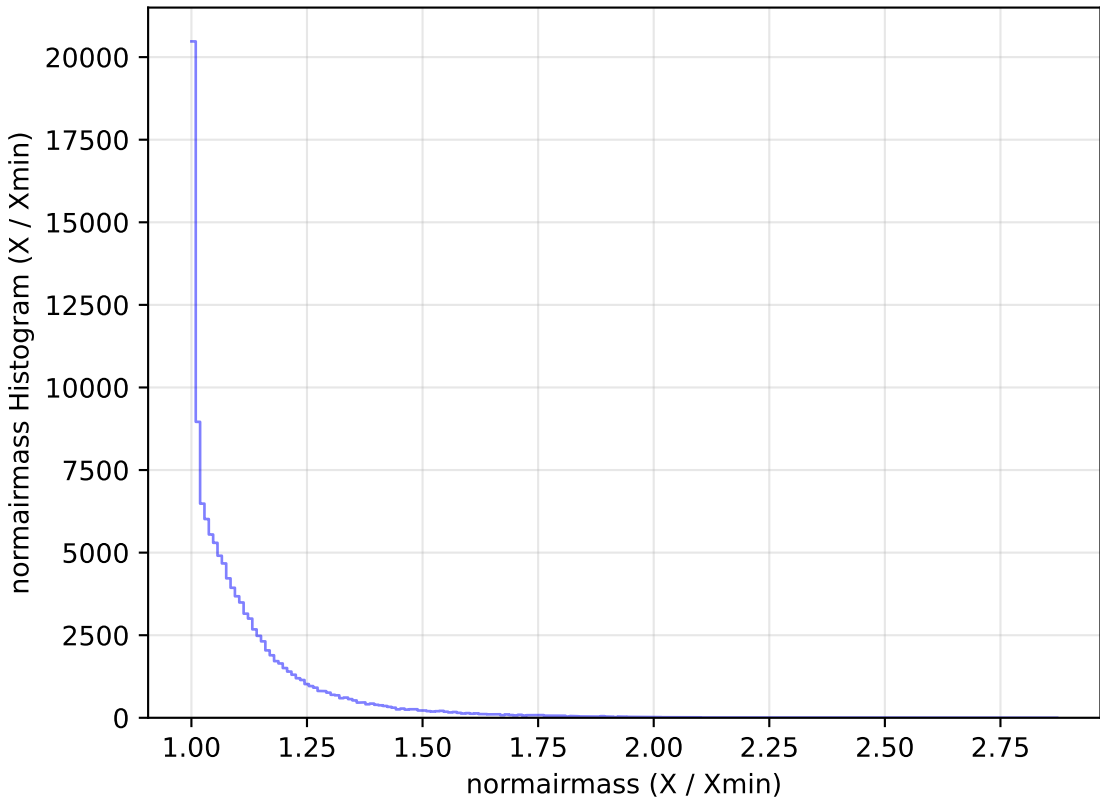
too_ignore_5_1v3.4_10yrs WFD u band: normairmass Histogram
