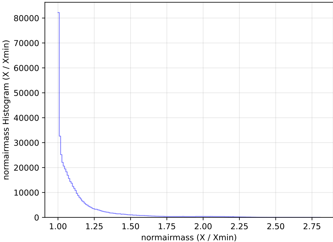
too_ignore_5_1v3.4_10yrs WFD r band: normairmass Histogram
