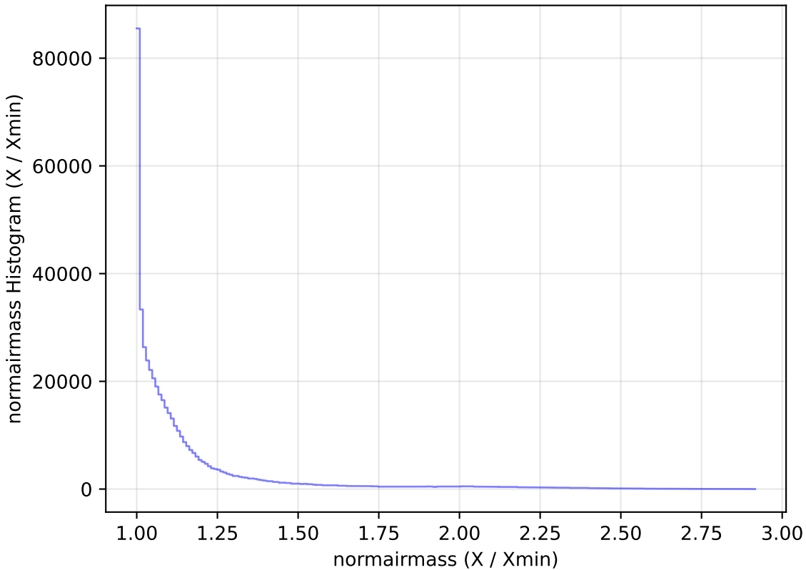
too_ignore_5_1v3.4_10yrs WFD i band: normairmass Histogram
