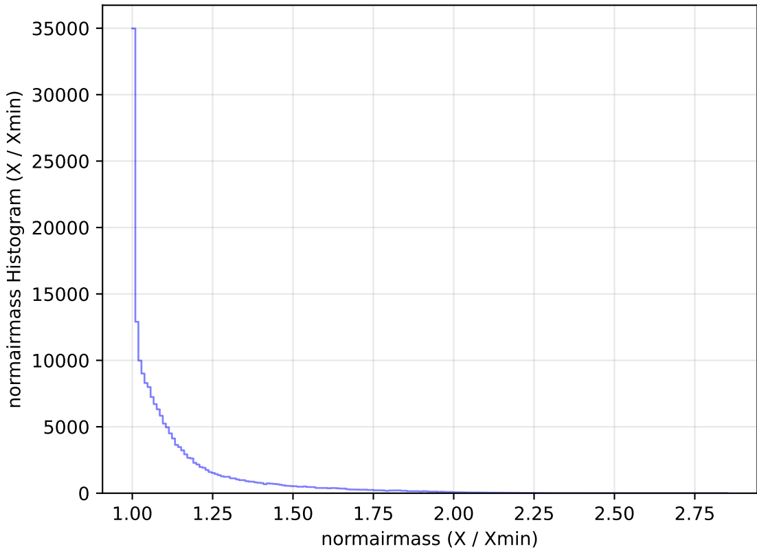
too_ignore_5_1v3.4_10yrs WFD g band: normairmass Histogram
