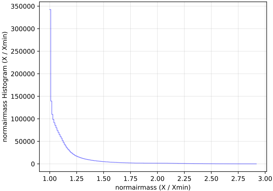
too_ignore_5_1v3.4_10yrs WFD all bands: normairmass Histogram
