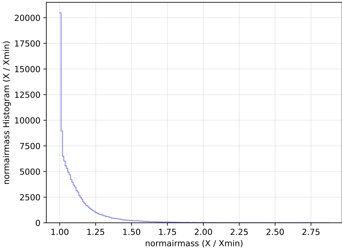
too_ignore_5_1v3.4_10yrs All sky u band: normairmass Histogram
