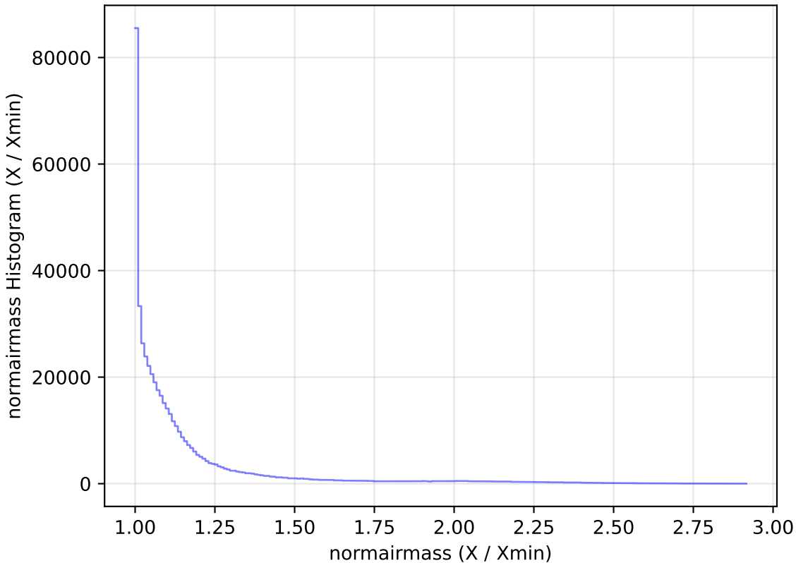
too_ignore_5_1v3.4_10yrs All sky i band: normairmass Histogram
