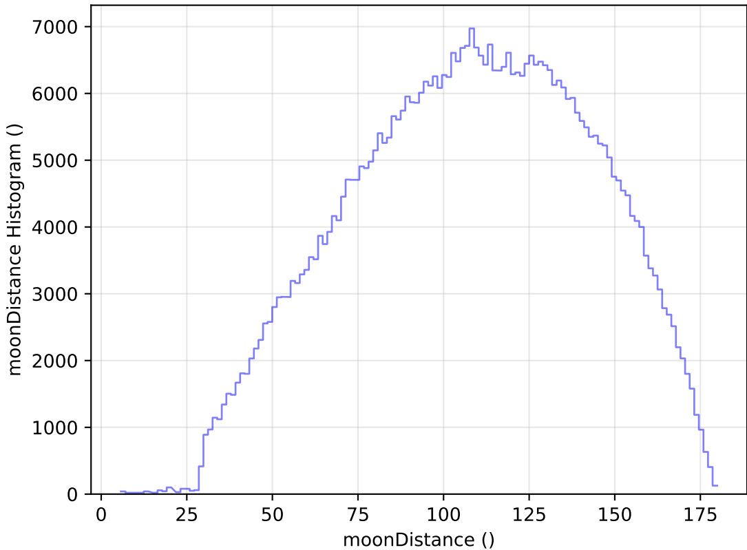
too_ignore_5_1v3.4_10yrs WFD r band: moonDistance Histogram
