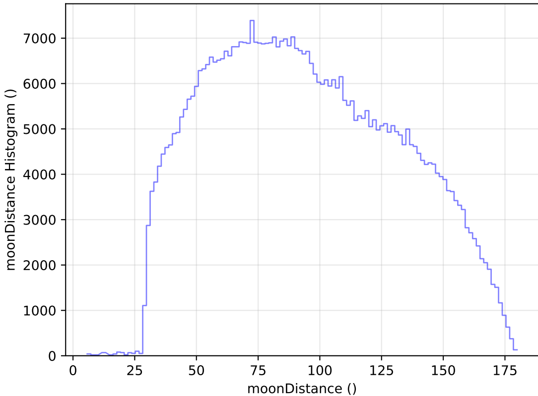
too_ignore_5_1v3.4_10yrs WFD i band: moonDistance Histogram
