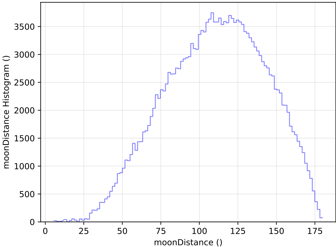
too_ignore_5_1v3.4_10yrs WFD g band: moonDistance Histogram
