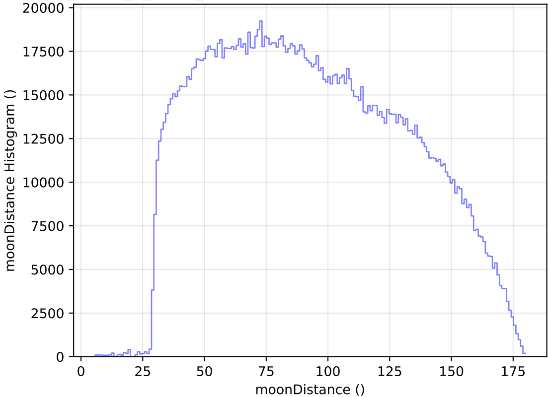
too_ignore_5_1v3.4_10yrs WFD all bands: moonDistance Histogram
