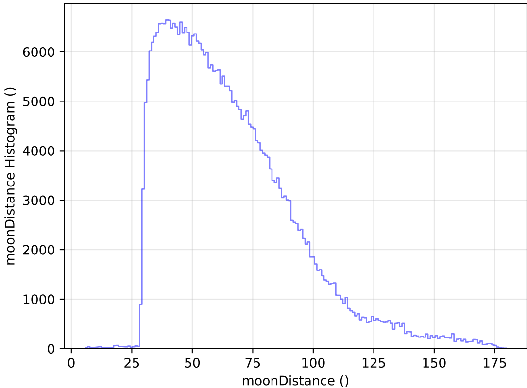
too_ignore_5_1v3.4_10yrs All sky y band: moonDistance Histogram
