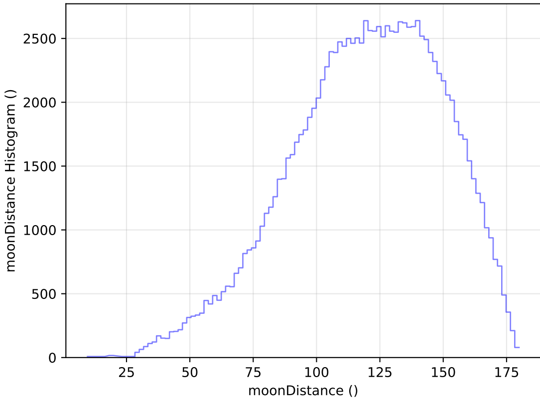
too_ignore_5_1v3.4_10yrs All sky u band: moonDistance Histogram
